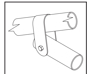
Cross Brace Strap
